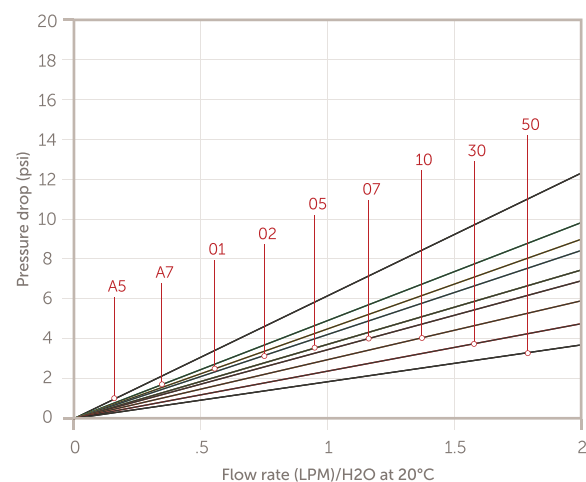
Planarcap NMB 2.5" Disposable Filters with 1/4" Inlet/Outlet Fitting (Ø89 mm)
