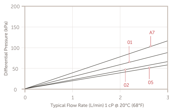
Planarcap NMB 2.5" Disposable Filters with 1/4" Inlet/Outlet Fitting (Ø73 mm)
