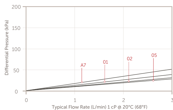
Planarcap NMB 5" Disposable Filters with 1/4" Inlet/Outlet Fitting (Ø73 mm)
