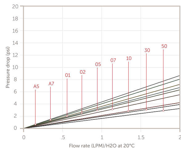
Planarcap NMB 5" Disposable Filters with 1/4" Inlet/Outlet Fitting (Ø89 mm)
